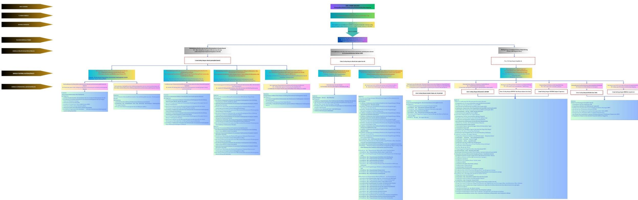
Gambar 3.1 Cascading
